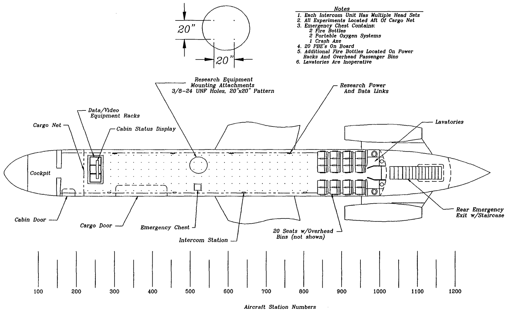
Figure 2. - Overhead view of DC-9
