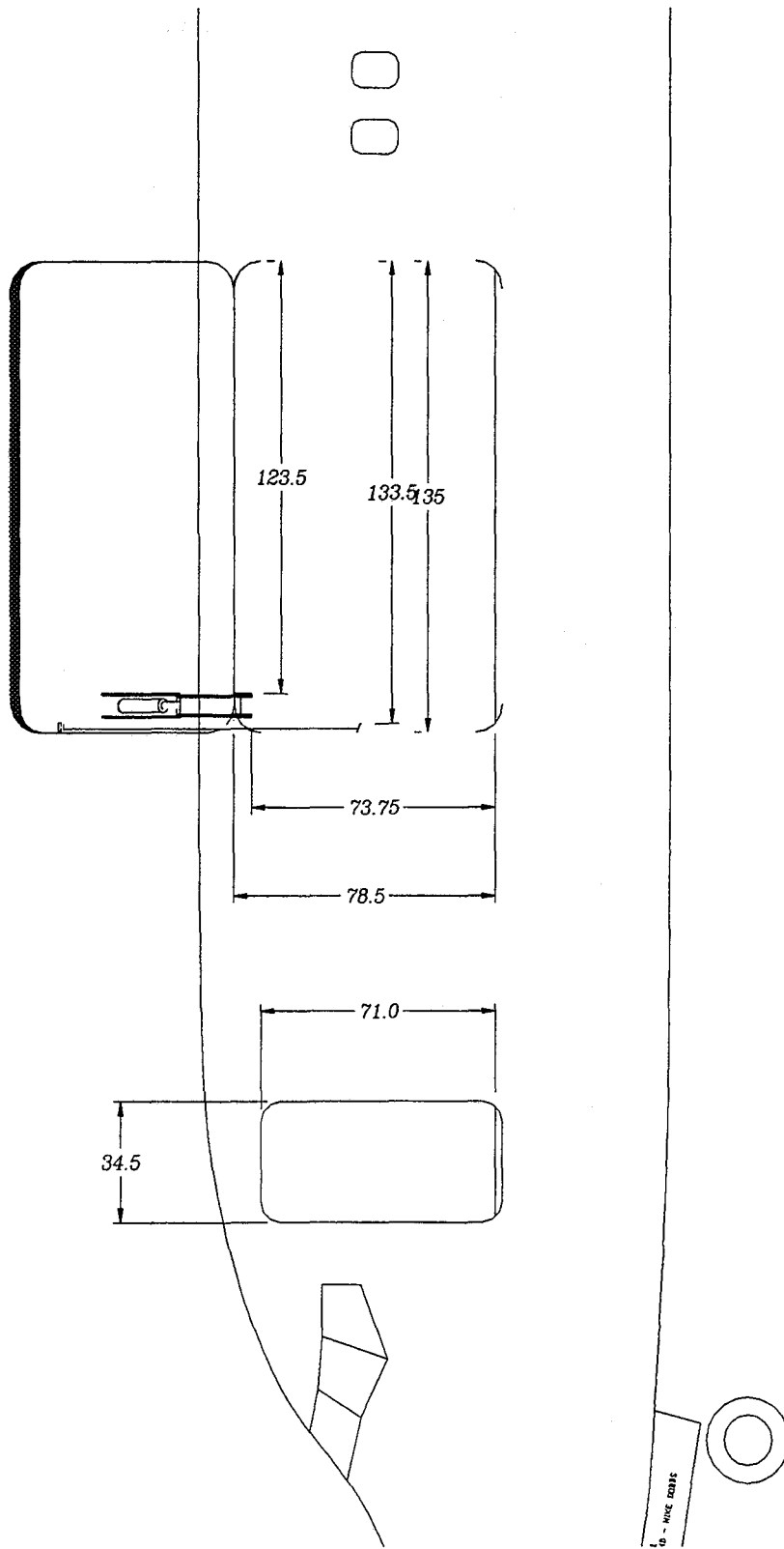
Figure 4. - DC-9 Cargo door usable opening (Dimensions are in inches.)
