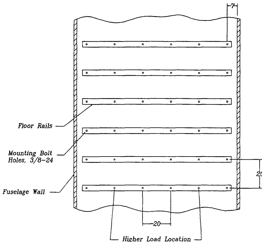
Aircraft Floor, Top View Detail Drawing Indicating Load Limitations On Floor Rails
