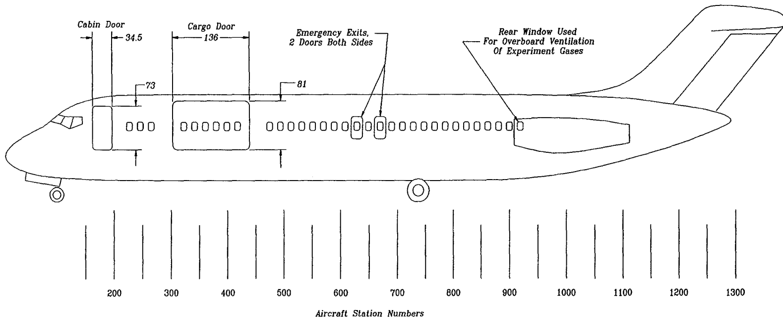
Figure 3. - Side view of DC-9 (Dimensions are in inches.)
